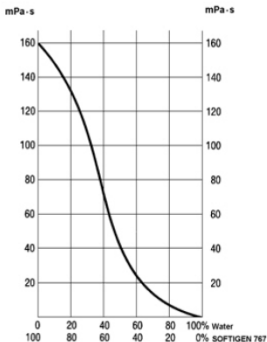
figure 2) Viscosity of aqueous in SOFTIGEN® 767 mixtures
