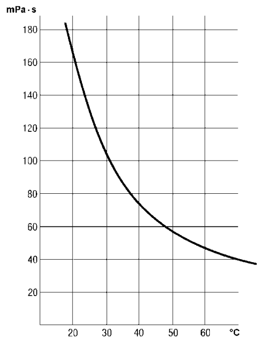
figure 1) Viscosity of SOFTIGEN® 767 relation to temperature
